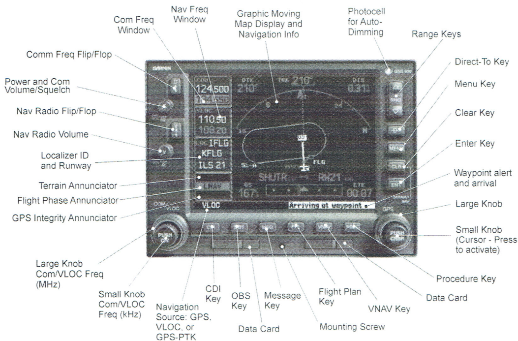
Figure 1 - 530W Series Control and Display Layout
